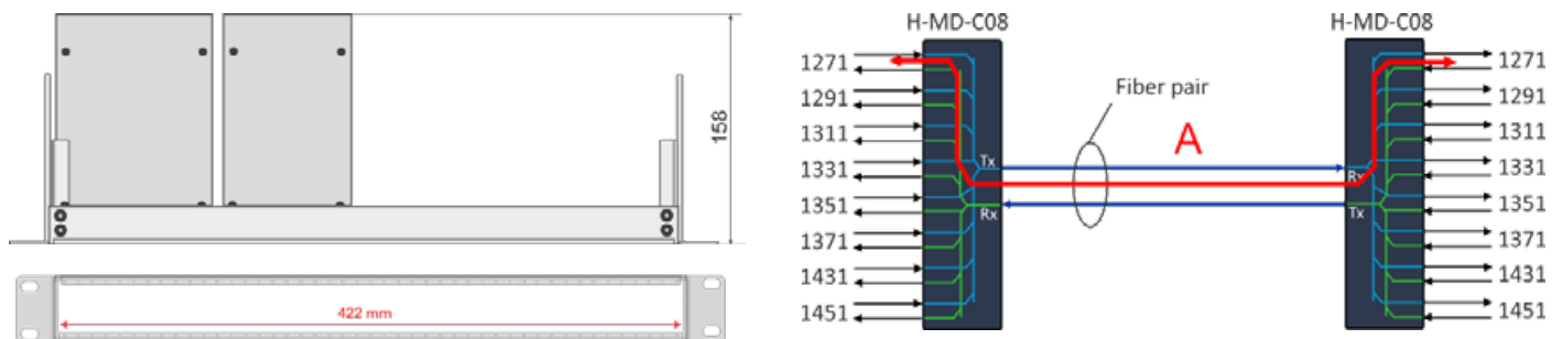
Mounting bracket dimensions with two example filters.
